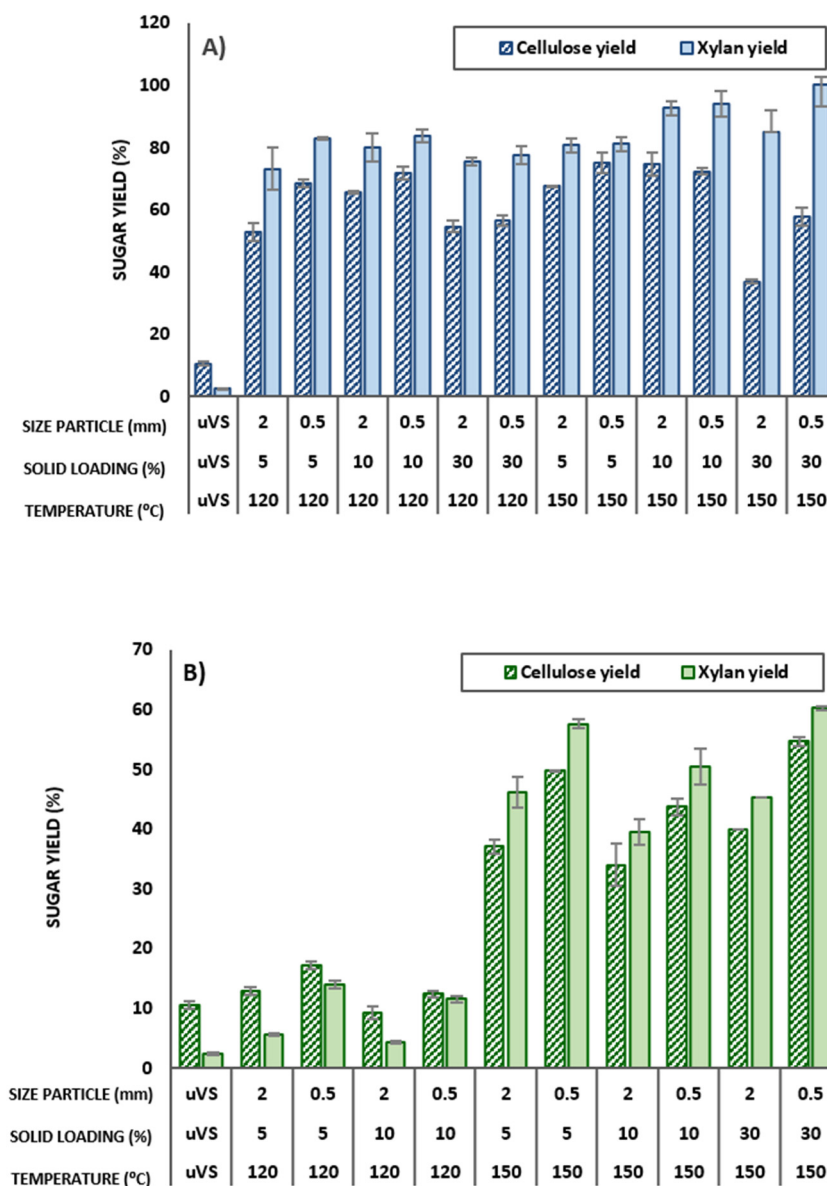
Figure 4. Effect of pretreatment conditions on conversion yield (cellulose and xylan yield (%) calculated by Equation (3) and Equation (4), respectively) after enzymatic hydrolysis of DES-pretreated vine shoots with (A) ChCl:LA (1:5) and (B) ChCl:EG (1:2). uVS = untreated VS biomass.
