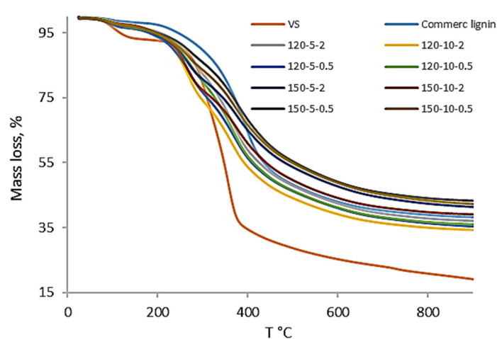
Figure 5. Evolution of the mass loss (g/100 g dry biomass, (%)) of the raw VS biomass, commercial lignin, and the solids S2 at different ChCl:LA (1:5) pretreatment conditions versus temperature (°C).
