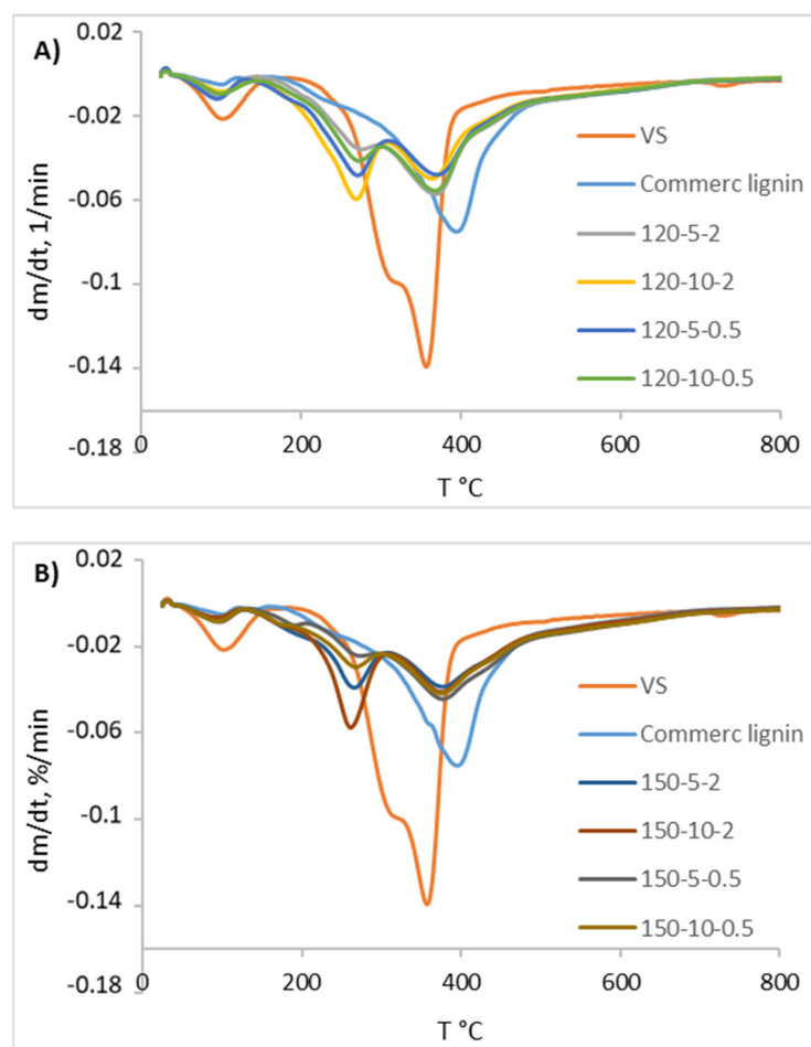
Figure 6. Differential thermogravimetric analysis (DTG) profiles obtained for the samples of ChCl:LA lignin-enriched solids generated at different conditions of solid load and particle size: (A) 120 °C; (B) 150 °C.
