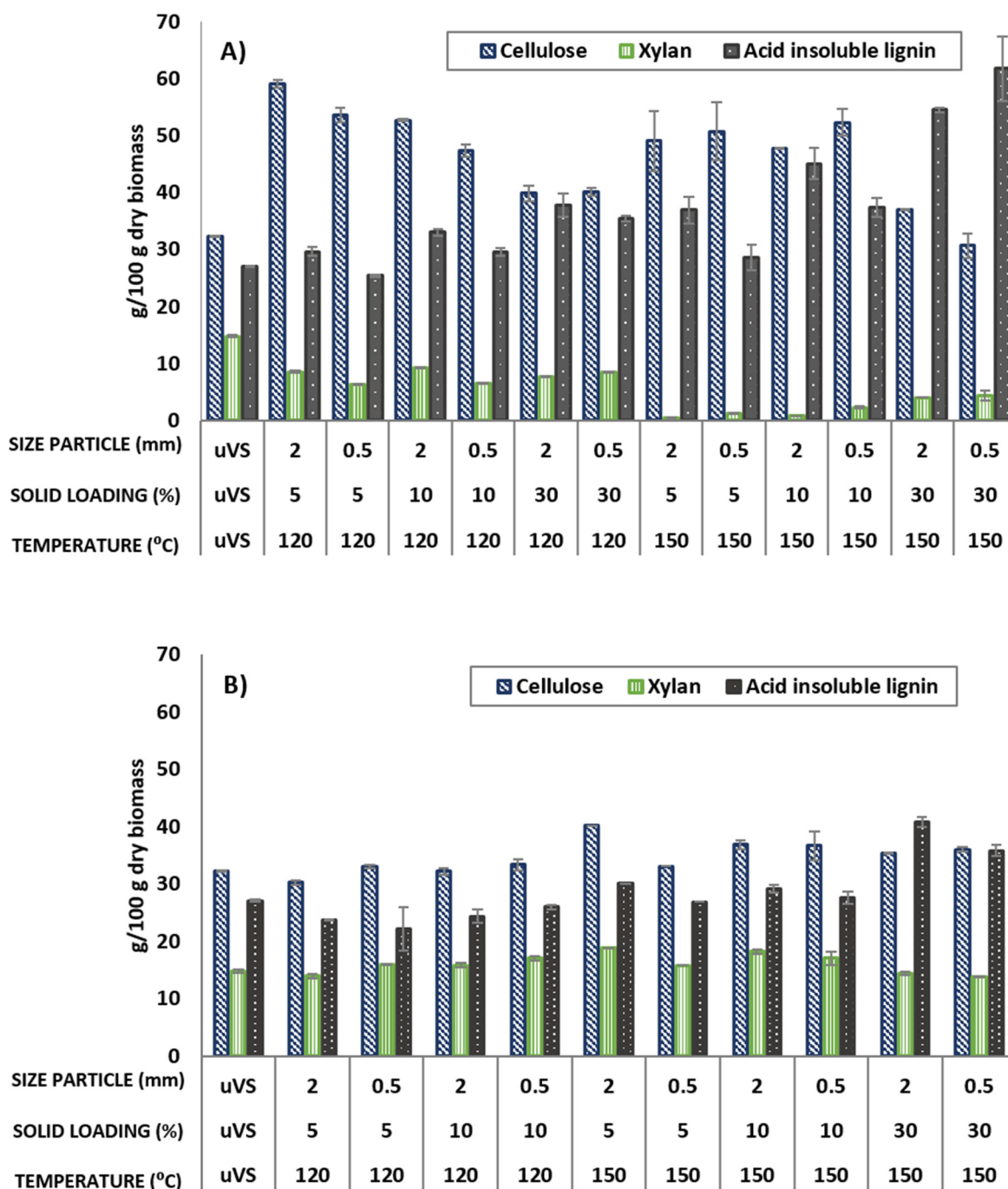
Figure 2. Main components: cellulose, xylan, and acid-insoluble lignin (calculated as g/100 g of dry biomass, (%) of the solid residues pretreated using different DESs: (A) ChCl:LA (1:5) and (B) ChCl:EG (1:2). uVS = untreated VS biomass.
