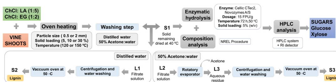
Figure 1. Schematic diagram of solvent pretreatment in this study. Abbreviations and nomenclature definition: ChCl: LA, choline chloride/lactic acid; ChCl:EG, choline chloride/ethylene glycol; S1, solid sample after pretreatment and washing step; L1, filtrate solution with distilled water; L2, filtrate solution with 50% acetone/water; L3, aqueous residue; S2, lignin-enriched solid after water washing; S3, lignin-enriched solid after 50% acetone/water washing.
